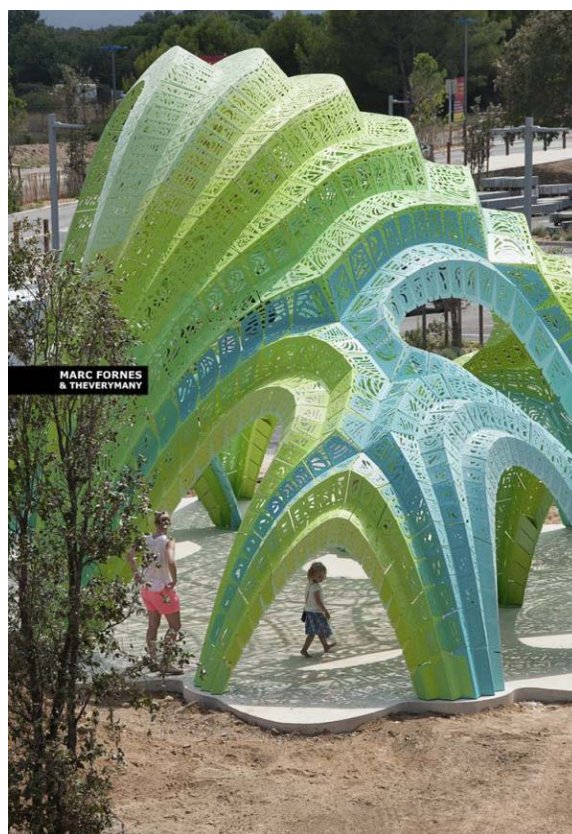
134. Pleated Inflation | Informal amphitheater | Argeles-Sur-Mer, France | 2013 Design & computation: MARC FORNES / THEVERYMANY Location: Lycee Christian Bourquin, Argeles-Sur-Mer Hypothesis of research: self-supported shell through pleated inflation + agents based porosity (implementing our Calder installation) Photos series: "end assembly" v.150828: Fuente: https://theverymany.com/public-art/argeles-sur-mer/
