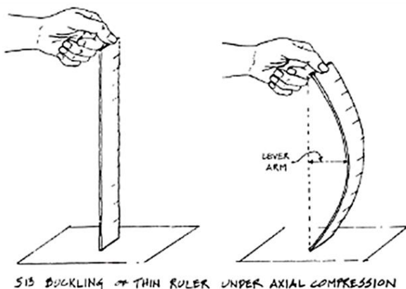
513 BUCKLING OF THIN RULER UNDER AXIAL COMPRESSION
